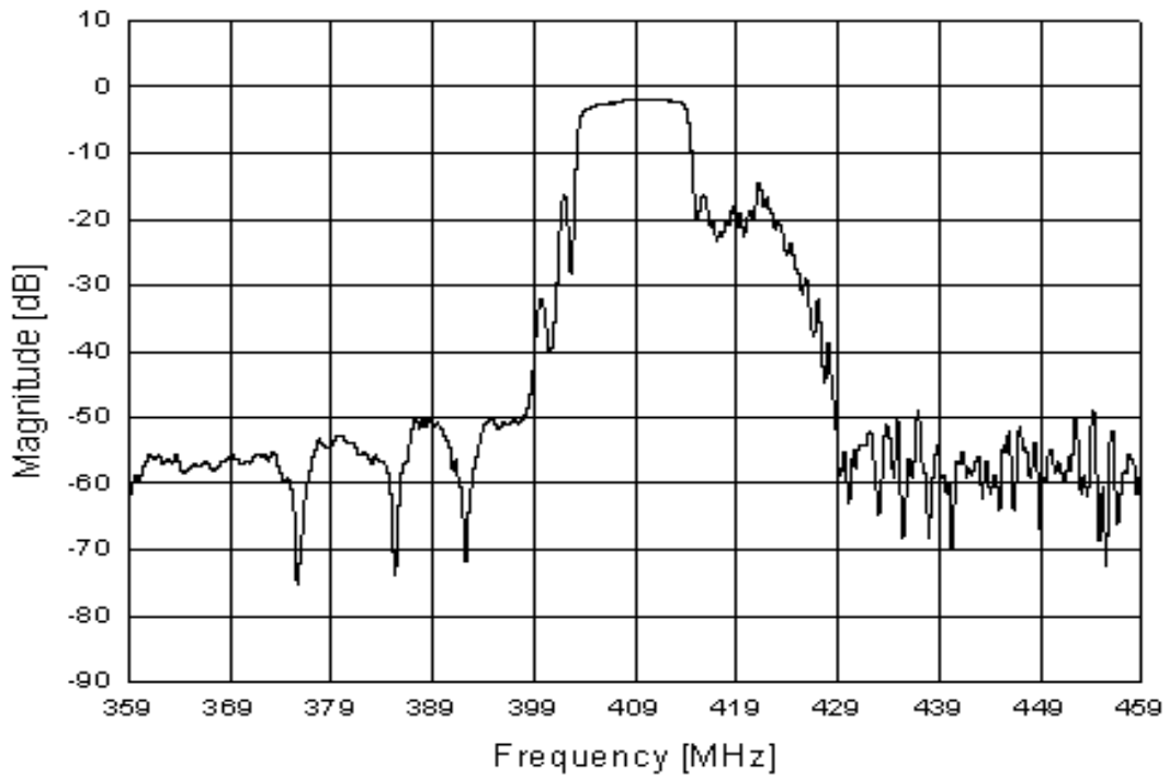
Frequency Response
